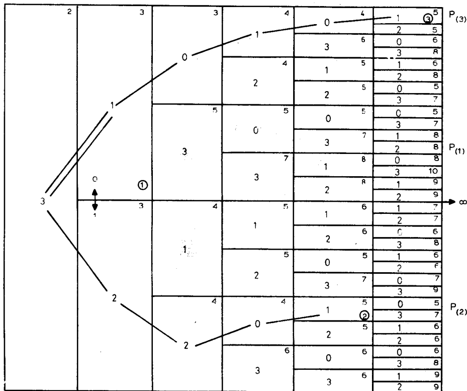
Fig. 3 Selection of permissible paths from the lower-half initial code tree
