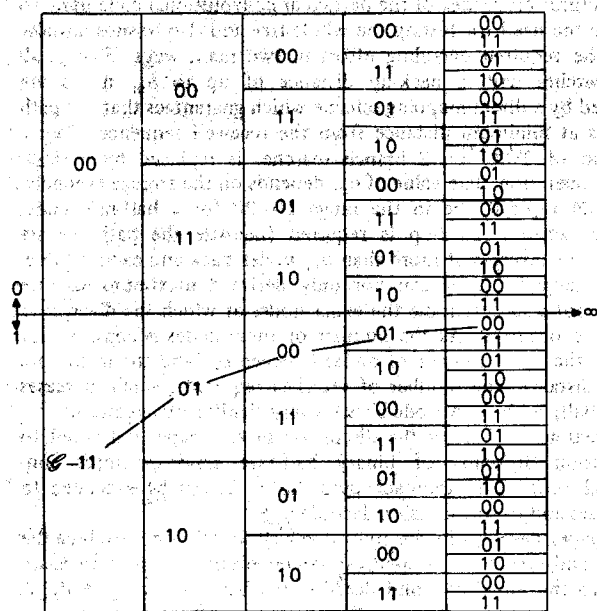
Fig. 2 The development of the initial code tree for the half-rate code with \mathcal{G} = 11 01 00 01 00 \dots g(2^{K-1})
