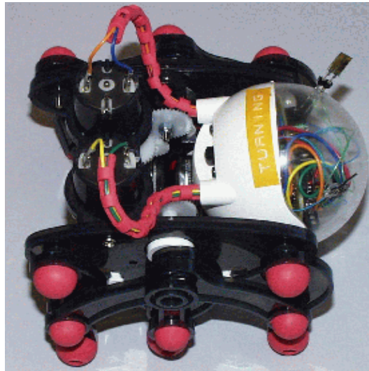
Figure 5: This robot, built from a toy kit produced by the Elekit company, contains only two sensors oriented at a 90^\circ from each other, with their mid-angle located along the robot's apparent line of motion. The robot is powered by two DC motors, each controlling one set of 'legs', and has a simple combinatorial logic controlling these motors.
